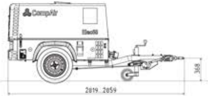
straight towbar, braked
